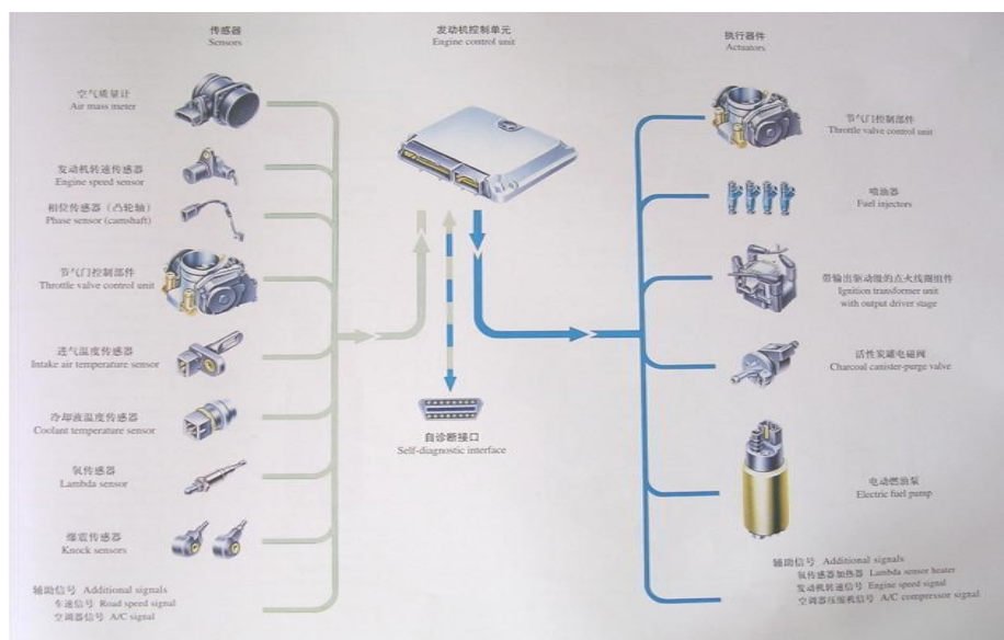
Sensor connection example diagram (as shown below) ▼
